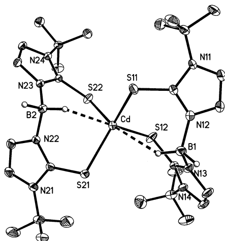
Figure 4. Molecular structure of Cd[Bm tBu ] 2 . Selected bond lengths (Å) and angles (deg): Cd–S(11) 2.5407(9), Cd–S(12) 2.5646(9), Cd–S(21) 2.5356(8), Cd–S(22) 2.5954(8), Cd···H(1) 2.73(3), Cd···H(4) 2.49(3), S(11)–C(11) 1.732(3), S(12)–C(18) 1.718(3), S(21)–C(21) 1.719(3), S(22)–C(28) 1.716(3); S(11)–Cd–S(12) 111.87(3), S(11)–Cd–S(22) 114.13(3), S(12)–Cd–S(22) 85.12(3), S(21)–Cd–S(11) 116.44(3), S(21)–Cd–S(22) 114.30(3), S(21)–Cd–S(12) 110.83(3), H(4)–Cd–S(21) 72.2(7), H(4)–Cd–S(11) 76.3(7), H(4)–Cd–S(12) 167.0(7), H(4)–Cd–S(22) 82.2(7), S(21)–Cd–H(1) 78.9(6), S(11)–Cd–H(1) 67.1(6), S(12)–Cd–H(1) 77.7(6), S(22)–Cd–H(1) 161.4(7), H(4)–Cd–H(1) 115.2(9).
