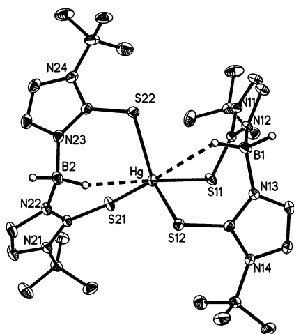
Figure 5. Molecular structure of Hg[Bm tBu ] 2 . Selected bond lengths (Å) and angles (deg): Hg–S(11) 2.5919(8), Hg–S(12) 2.5557(7), Hg–S(21) 2.5526(7), Hg–S(22) 2.5374(7), Hg···H(1) 3.09(3), Hg···H(4) 2.62(3), S(11)–C(11) 1.735(3), S(12)–C(18) 1.736(3), S(21)–C(21) 1.723(3), S(22)–C(28) 1.730(3); S(22)–Hg–S(21) 112.23(3), S(22)–Hg–S(12) 110.50(2), S(21)–Hg–S(12) 123.89(3), S(22)–Hg–S(11) 112.94(3), S(21)–Hg–S(11) 94.77(2), S(12)–Hg–S(11) 100.40(3), S(22)–Hg–H(4) 70.4(6), S(21)–Hg–H(4) 79.0(6), S(12)–Hg–H(4) 82.8(6), S(11)–Hg–H(4) 173.8(6), S(22)–Hg–H(1) 66.3(5), S(21)–Hg–H(1) 174.2(5), S(12)–Hg–H(1) 61.1(5), S(11)–Hg–H(1) 81.0(5), H(4)–Hg–H(1) 105.2(8).
